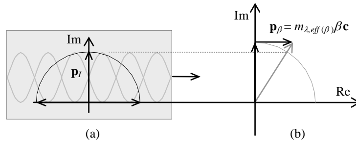
FIGURE 8-1. (a) The momentum of an electromagnetic resonator can be expressed in terms of an internal momentum \mathbf{p}_I of the standing wave in the resonator frame and (b) the external momentum \mathbf{p}_\beta of the resonator as an energy object moving at velocity v = c \cdot \beta in the parent frame.
