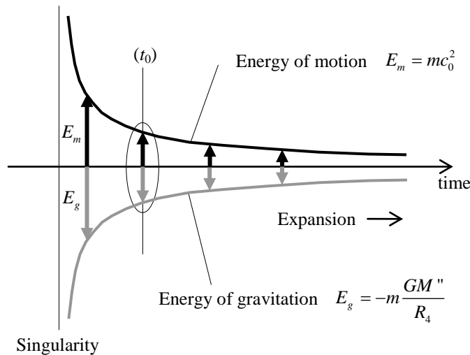
FIGURE 1-2. The dualistic expression of the rest energy of matter. In the expansion of space the rest energy gained in a pre-singularity contraction phase is gradually released back to the gravitational energy. The zero-energy linkage of the complementary expressions of energy links any localized mass object to the rest of space.
