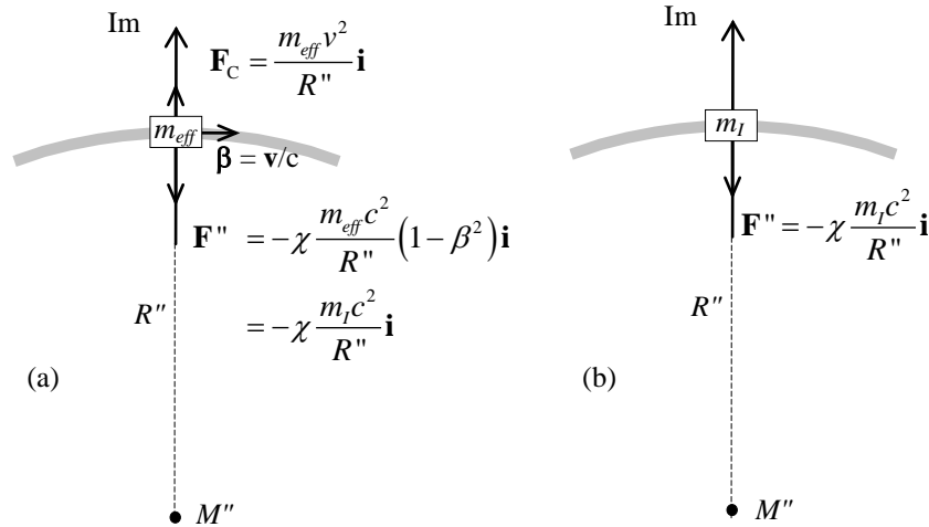
FIGURE 4-4. (a) The gravitational force of mass equivalence M'' on mass m_{eff} moving at velocity \mathbf{v} with a local frame is reduced by the central force F_C , which makes it equal to the gravitational force of mass equivalence M'' on mass m_I at rest in the local frame as illustrated in figure (b).
