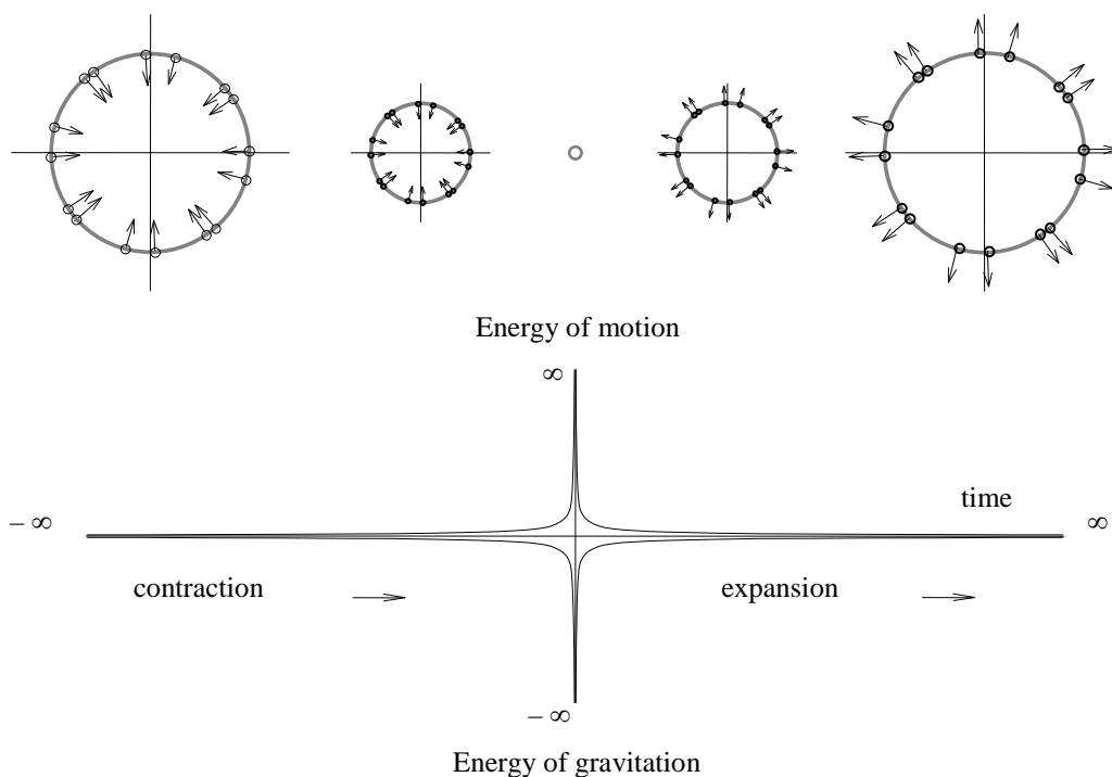
FIGURE 1-1. Energy buildup and release in spherical space. In the contraction phase, the velocity of space in the direction of the 4-radius increases due to the energy gained against loss of gravitation. In the expansion phase, the velocity gradually decreases, when the energy of motion gained in contraction is returned to gravity.
