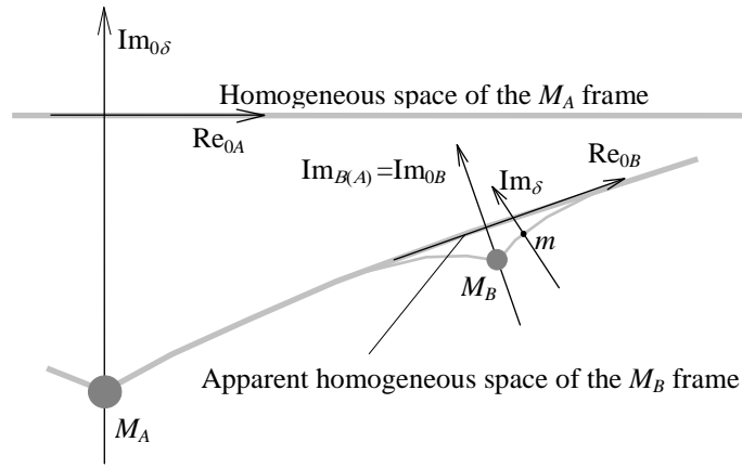
FIGURE 4-2. The apparent homogeneous space of the M_B -frame around mass center M_B follows the direction of space in the M_A -frame as it would be without the M_B center.
