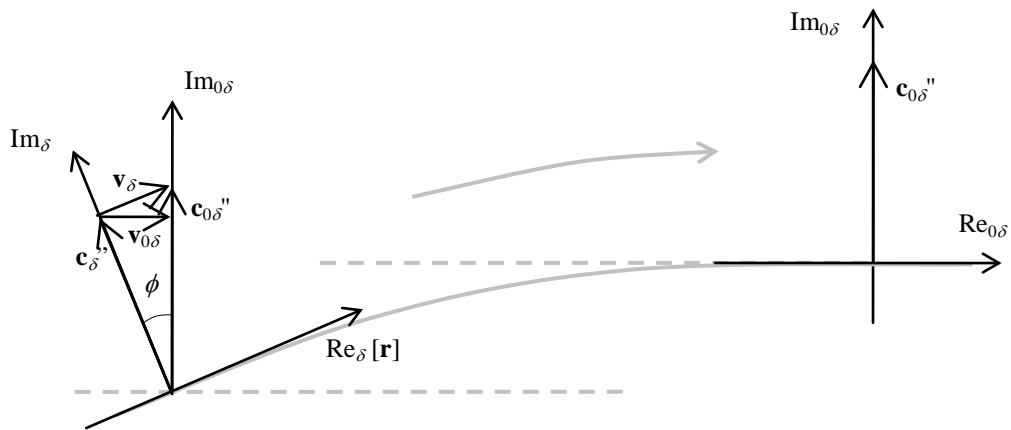
FIGURE 2-1. Escape velocity v_{0\delta} in the direction of the \text{Re}_0 axis is the velocity at which escape proceeds in the direction of the non-tilted space. Angle \phi approaches zero and velocity v_{0\delta} approaches velocity v_{\delta} when the escape approaches the non-tilted space. As illustrated in the figure, the momentum in equation (2.4:1) can be expressed as \mathbf{p}_{\delta}' = m v_{\delta} \hat{\mathbf{r}}_{\delta} of mass object m moving at velocity v_{\delta} in the local \delta -frame (in the direction of the \text{Re}_{\delta} axis) or momentum \mathbf{p}_{\delta}' = m' v_{0\delta} \hat{\mathbf{r}}_{\delta} of mass object m' = m / \sqrt{1 - \beta^2} = m / \cos \phi moving at velocity v_{0\delta} in homogeneous space frame (in the direction of the \text{Re}_0 axis). \beta = v_{\delta} / c_{0\delta} = v_{0\delta} / c_{\delta} = \sin \phi .
