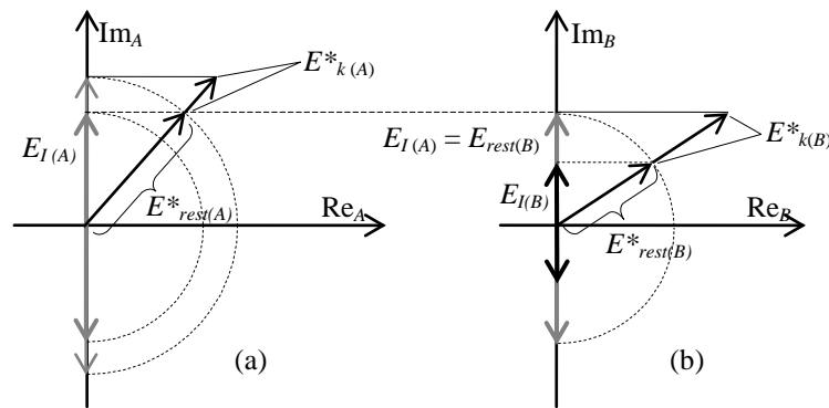
FIGURE 3-3. Kinetic energy (a) in frame A (the parent frame to frame B), and (b) in frame B moving in frame A. The internal energy E_{I(A)} of mass m in frame A appears as the rest energy mass has available in frame B. Accordingly, the kinetic energy E_{k(B)} of mass m in frame B is subject to the effects of motions both in frame B and the motion of frame B parent frame A.
