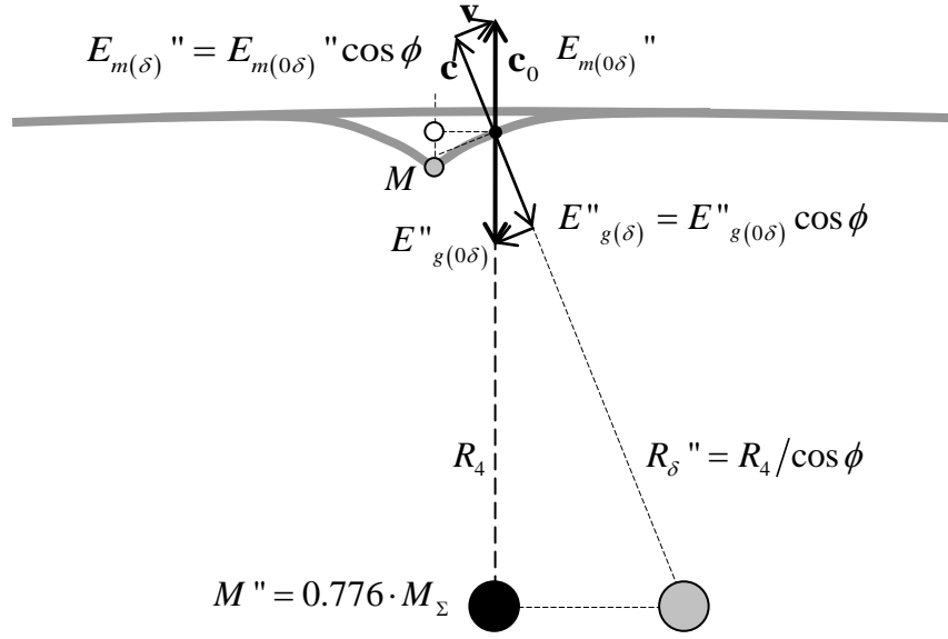
FIGURE 2-2. In tilted space ( M \ll M'' and R_\delta'' \ll R_4 ) the mass equivalence of homogeneous space appear in the direction of the local fourth dimension.
