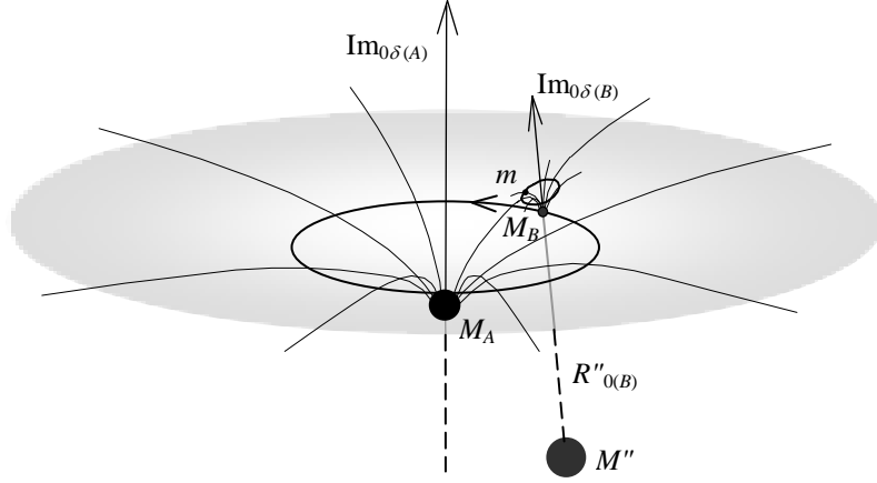
FIGURE 4-1. Mass object m rotating in the M_B gravitational frame rotates with the M_B -frame in the M_A -frame. Each mass center creates a local dent in space. Each dent in space reduces the local velocity of light and the motion of each frame reduces the mass of an object in a local frame.
