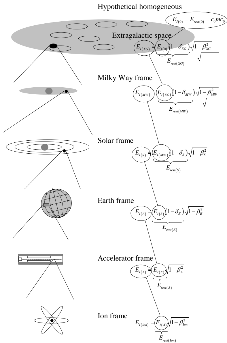
FIGURE 4-3. The rest energy of an object in a local frame is determined by the internal energy of the local frame in its parent frame. The internal energy is the imaginary component of the rest energy. The system of cascaded energy frames relates the rest energy of an object in a local frame to the rest energy of the object in hypothetical homogeneous space. As a consequence of the conservation of the total energy in space, motion and local gravitation of each parent frame reduce the rest energy available in the local frame.
